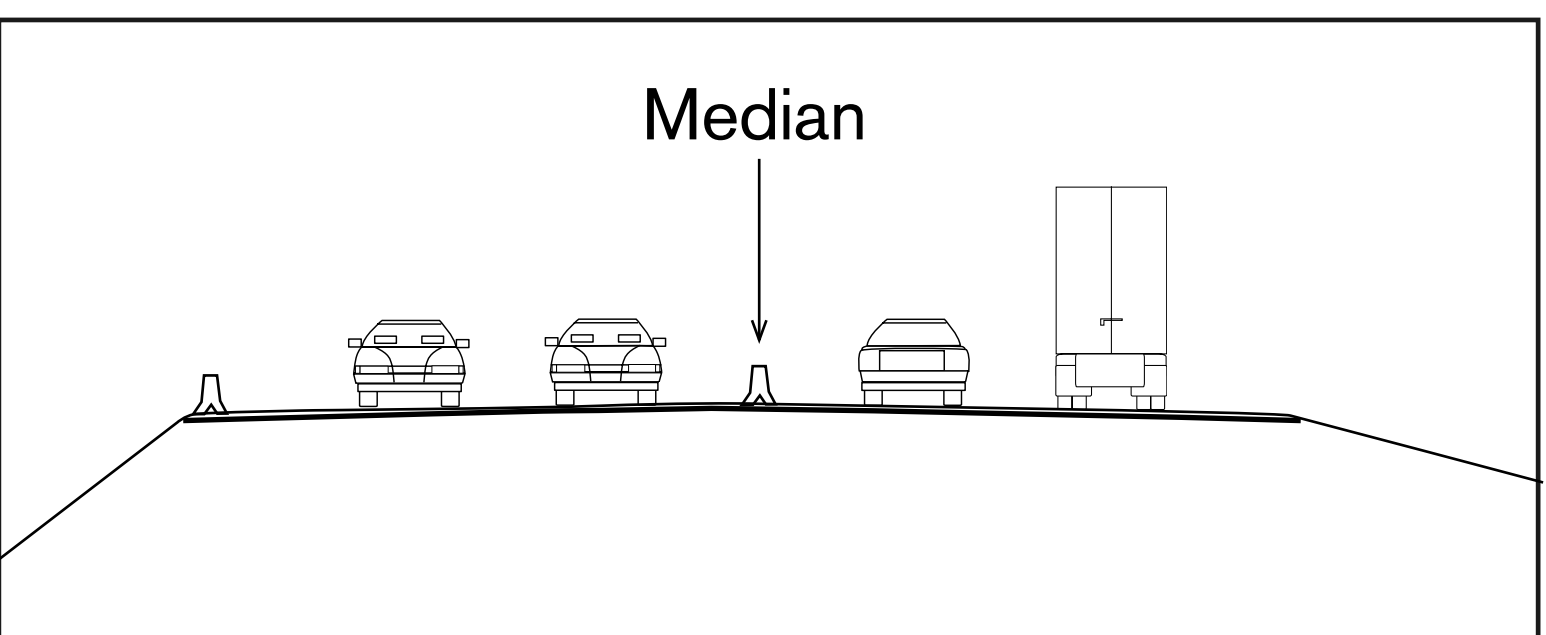
Typical Cross-Section
